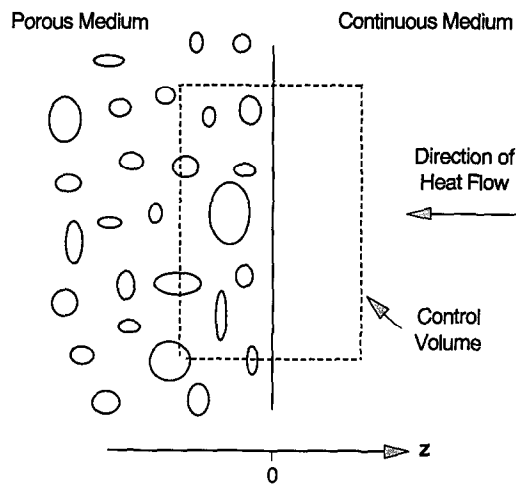
FIG. 1. Side view of a cylindrical control volume spanning the boundary between the porous and continuous media.
